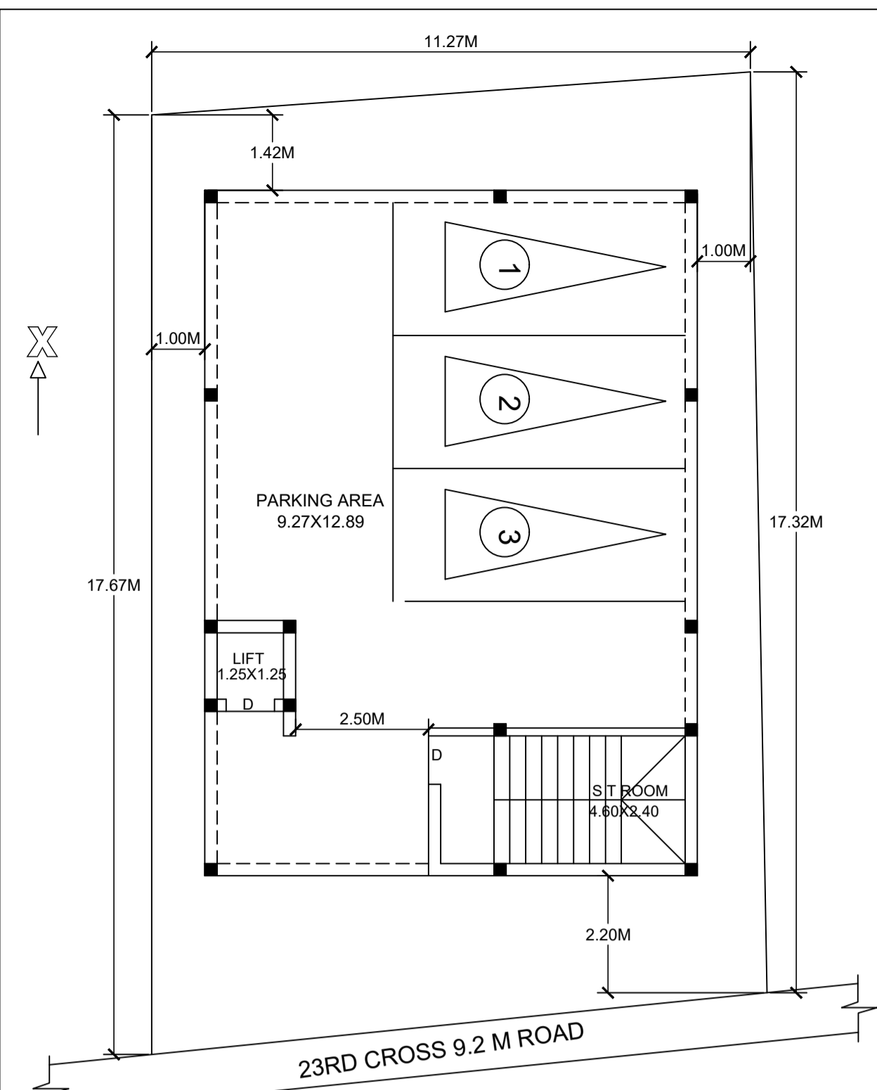
PROPOSED STILT FLOOR PLAN
